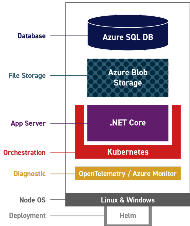
Figure 2—Aras Innovator Container Deployment
